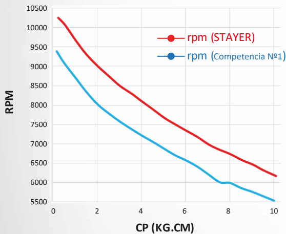
COMPARATIVA RPM VS TORQUE (Kg·cm)
