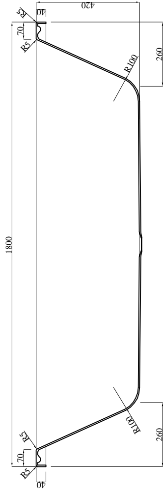
SECTION-A-A
