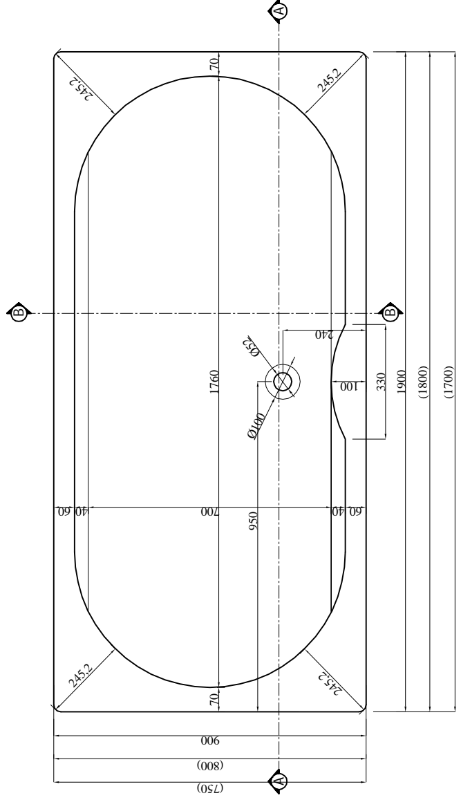
TOP VIEW
